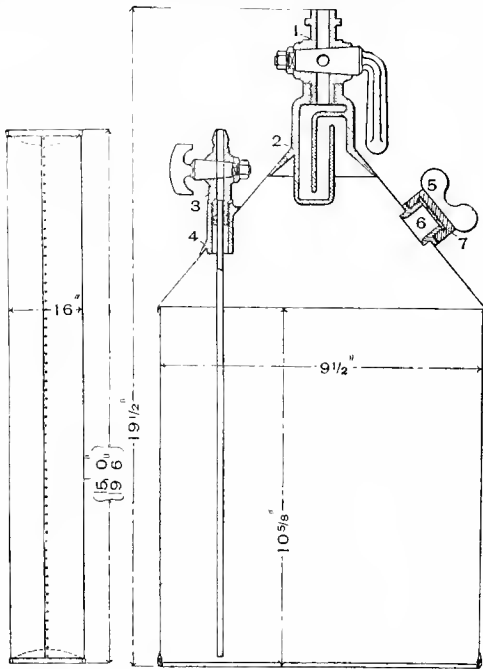
Fig. 3141. AIR-TANK.
